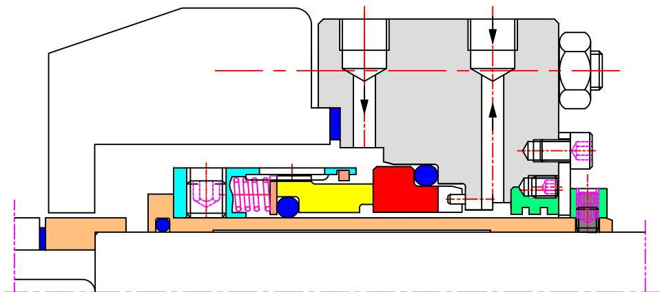
90 SERIES MULTI SPRINGS MECHANICAL SEAL TYPE 9101 CARTRIDGE ARRANGEMENT WITH DIFFERENT API PLAN 11& 62
